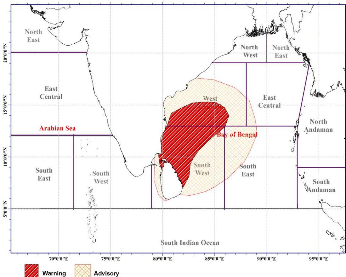
Advisory for Fishing and Naval Communities issued at 03.00 p.m. on 24 December 2022, valid for next 24 hours
