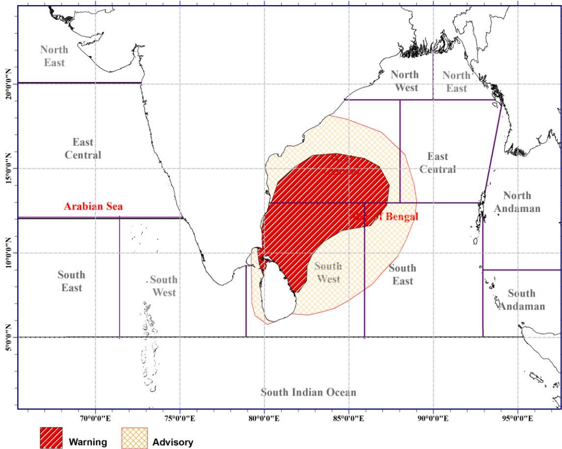
Advisory for Fishing and Naval Communities issued at 03.00 p.m. on 23 December 2022, valid for next 24 hours
